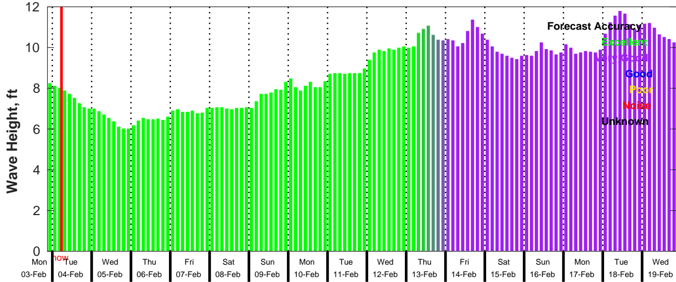
GFS Wave Forecast for NDBC 41040 from 03-Feb-2025 21:00:00 to 19-Feb-2025 21:00:00
