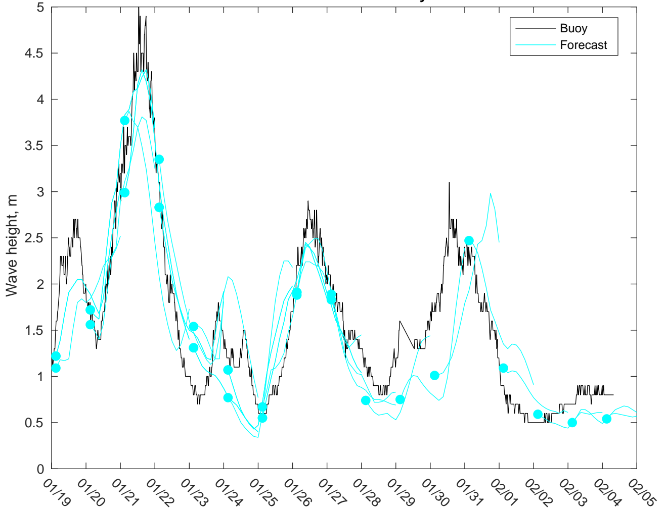
NDBC 42019 vs CMEMSWaves: 5 to 7 day forecast
