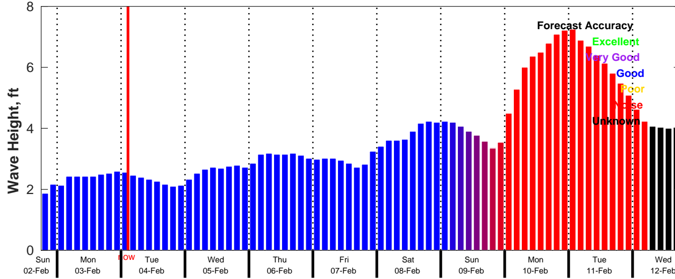
CMEMS Wave Forecast for NDBC 42019 from 02-Feb-2025 18:00:00 to 12-Feb-2025 18:00:00
