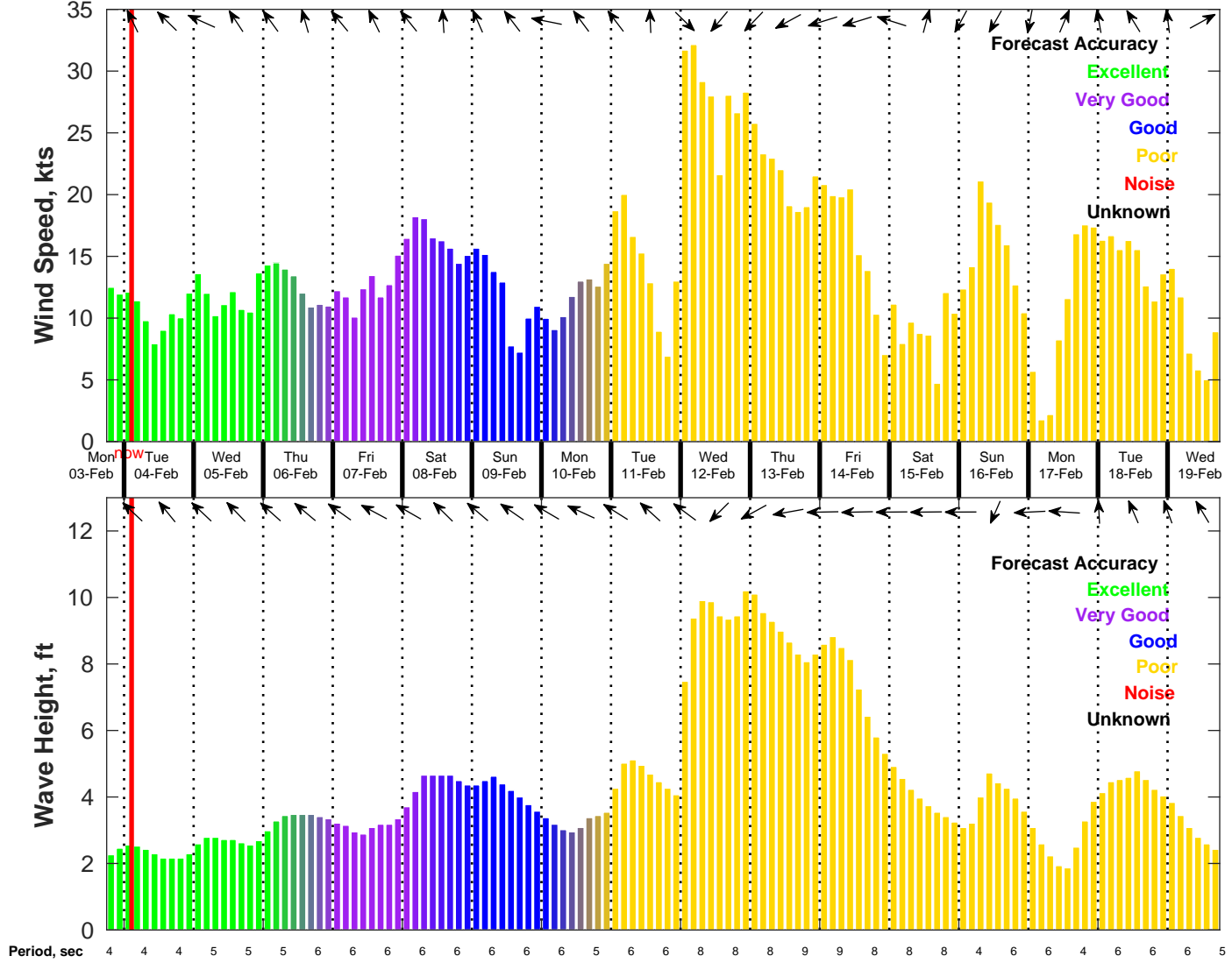
Wind & Wave Forecast for NDBC 42019 from 03-Feb-2025 18:00:00 to 19-Feb-2025 18:00:00
