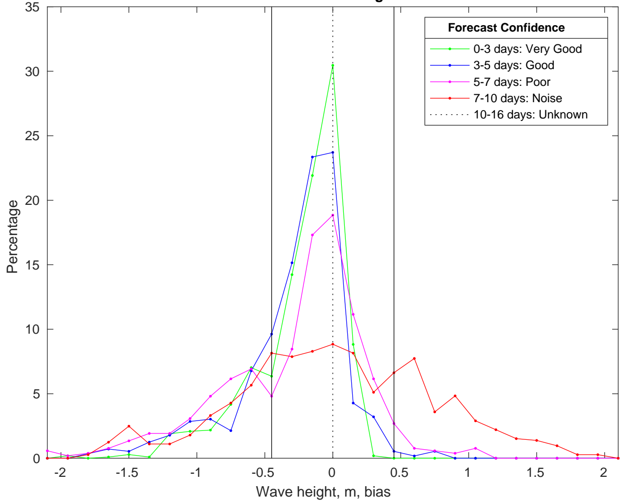
NDBC 42020 vs CMEMSWaves Bias Histogram: 04-Feb-2025
