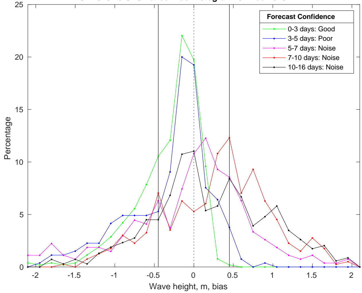
NDBC 42020 vs GFSWaves Bias Histogram: 04-Feb-2025
