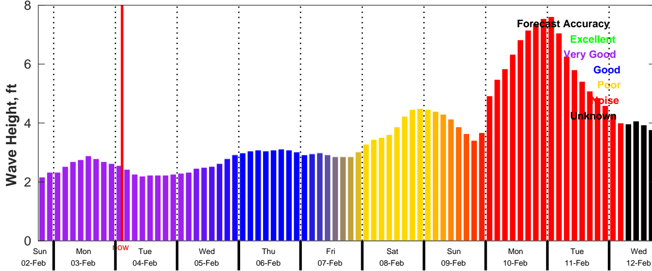
CMEMS Wave Forecast for NDBC 42020 from 02-Feb-2025 18:00:00 to 12-Feb-2025 18:00:00
