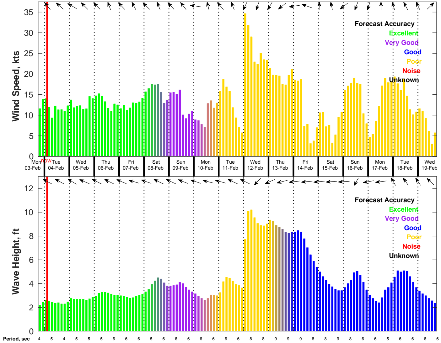
Wind & Wave Forecast for NDBC 42020 from 03-Feb-2025 18:00:00 to 19-Feb-2025 18:00:00
