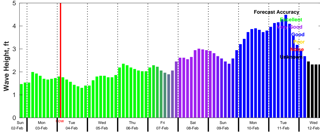
CMEMS Wave Forecast for NDBC 42035 from 02-Feb-2025 18:00:00 to 12-Feb-2025 18:00:00
