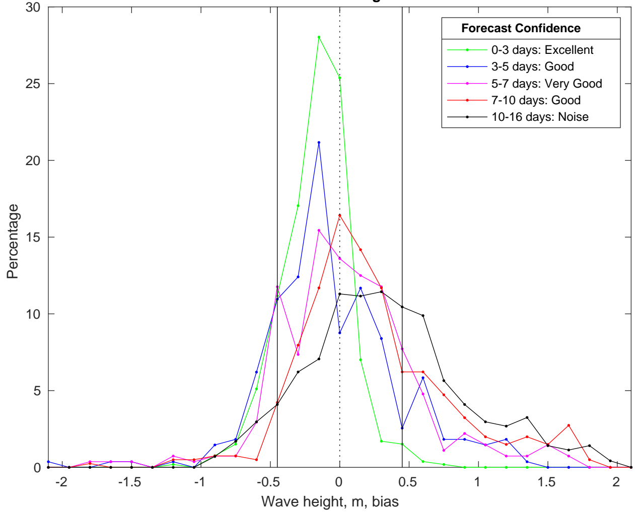
NDBC 42036 vs GFSWaves Bias Histogram: 04-Feb-2025
