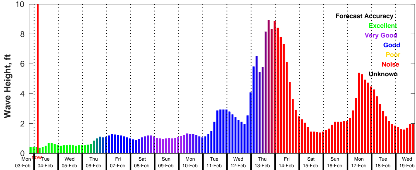
GFS Wave Forecast for NDBC 42036 from 03-Feb-2025 19:00:00 to 19-Feb-2025 19:00:00
