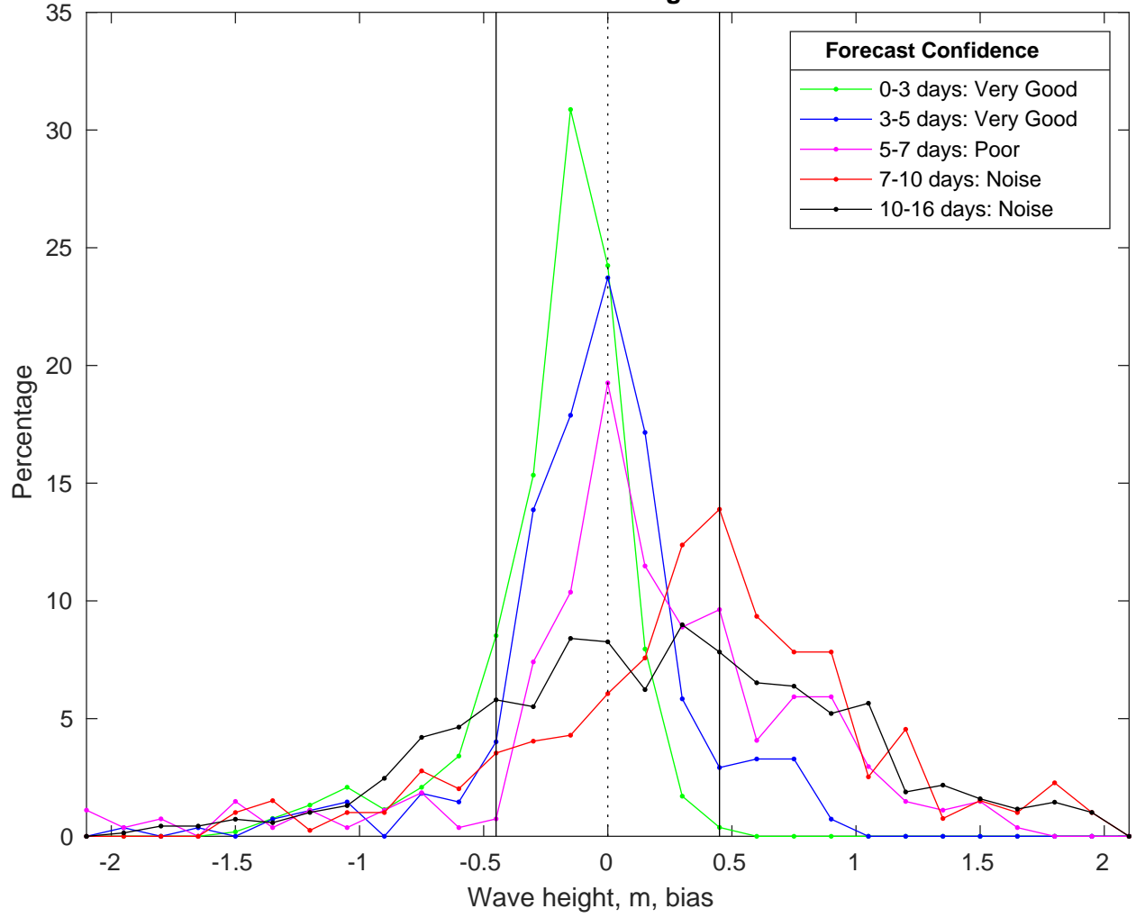
NDBC 42040 vs GFSWaves Bias Histogram: 04-Feb-2025
