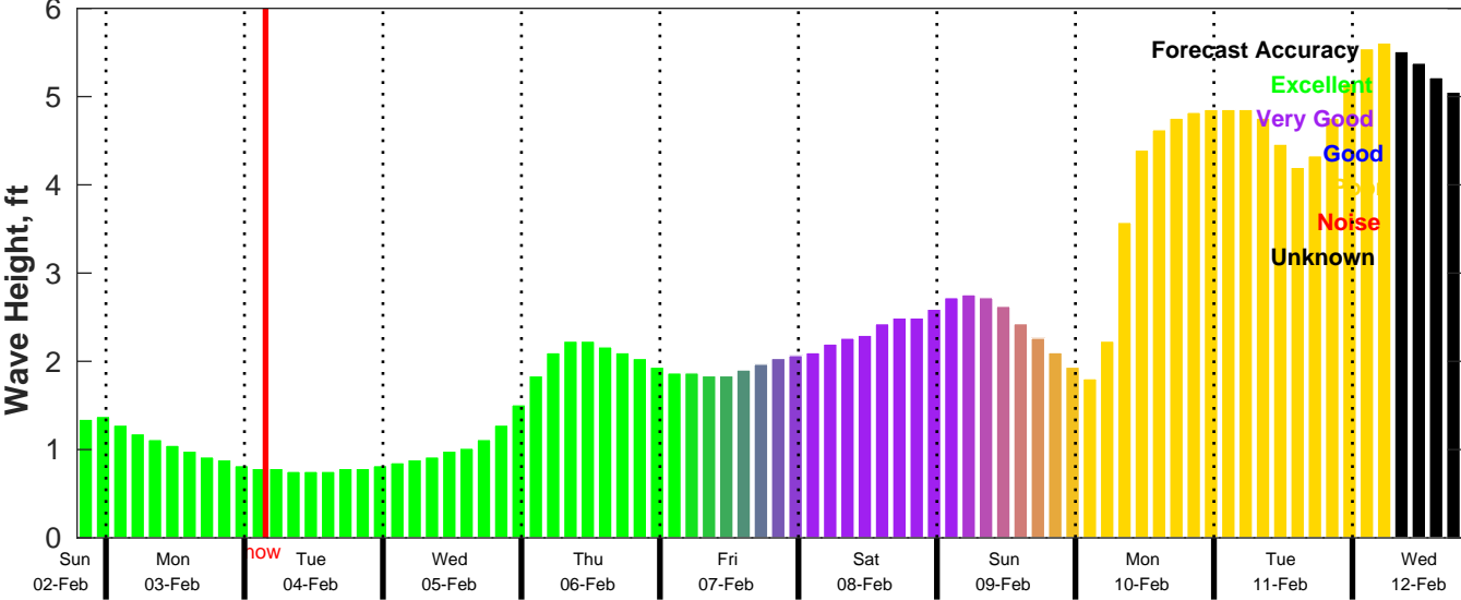
CMEMS Wave Forecast for NDBC 42040 from 02-Feb-2025 19:00:00 to 12-Feb-2025 19:00:00
