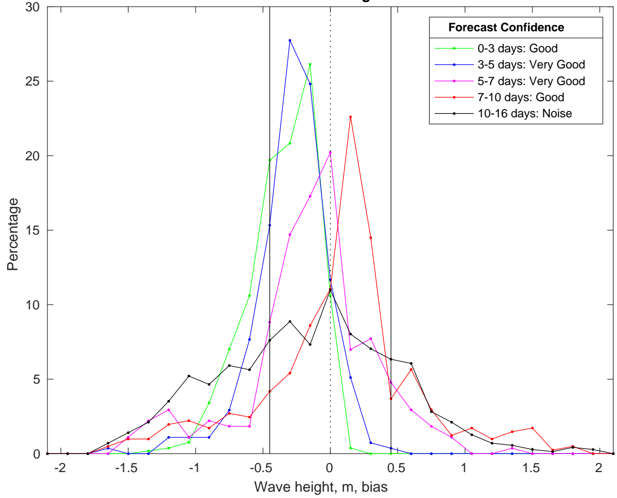
NDBC 42084 vs GFSWaves Bias Histogram: 04-Feb-2025
