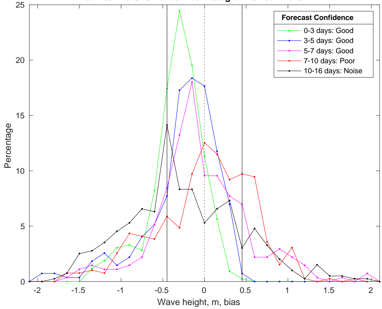
NDBC 42092 vs GFSWaves Bias Histogram: 31-Jan-2025
