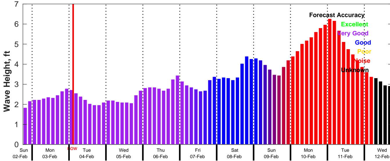
CMEMS Wave Forecast for NDBC 42092 from 02-Feb-2025 18:00:00 to 12-Feb-2025 18:00:00
