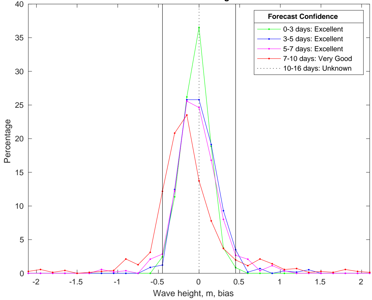
NDBC 46011 vs CMEMSWaves Bias Histogram: 04-Feb-2025
