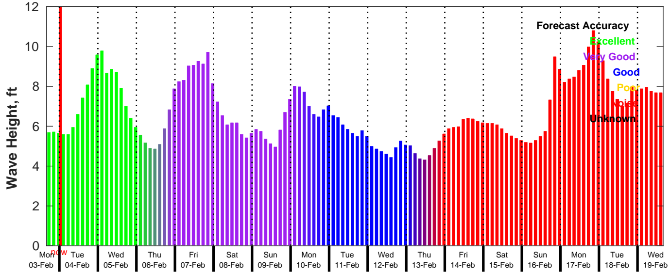
GFS Wave Forecast for NDBC 46011 from 03-Feb-2025 16:00:00 to 19-Feb-2025 16:00:00
