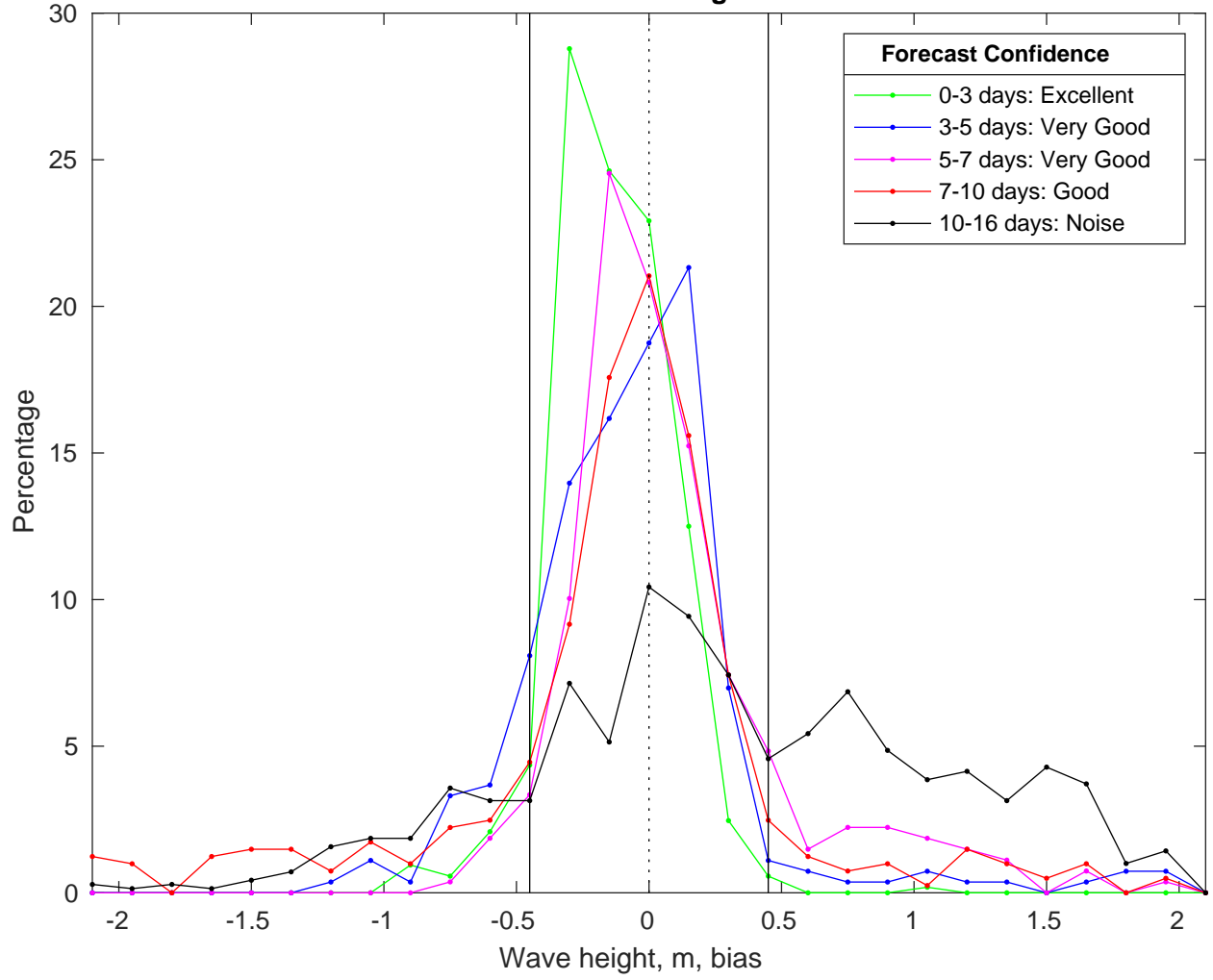
NDBC 46028 vs GFSWaves Bias Histogram: 04-Feb-2025
