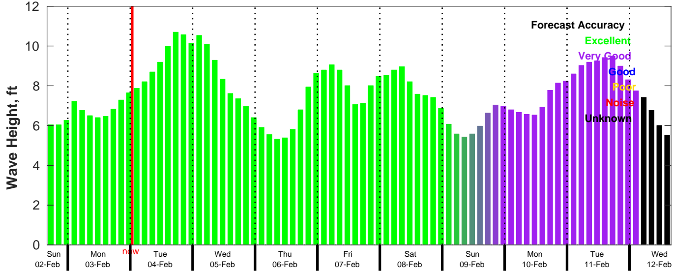
CMEMS Wave Forecast for NDBC 46028 from 02-Feb-2025 16:00:00 to 12-Feb-2025 16:00:00
