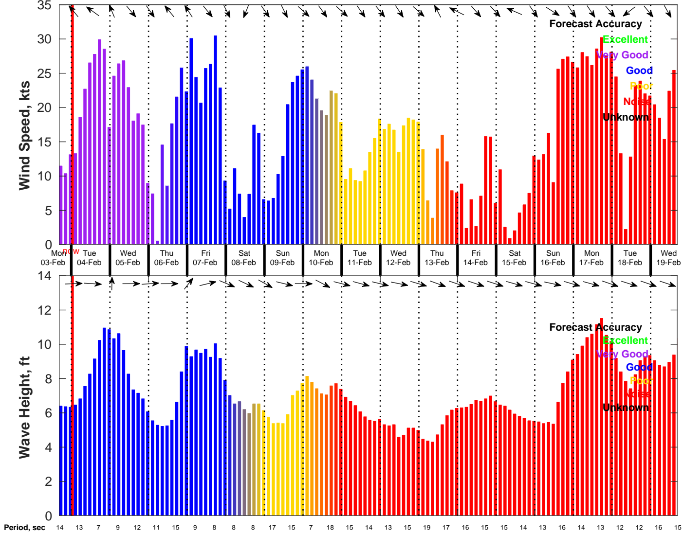
Wind & Wave Forecast for NDBC 46028 from 03-Feb-2025 16:00:00 to 19-Feb-2025 16:00:00
