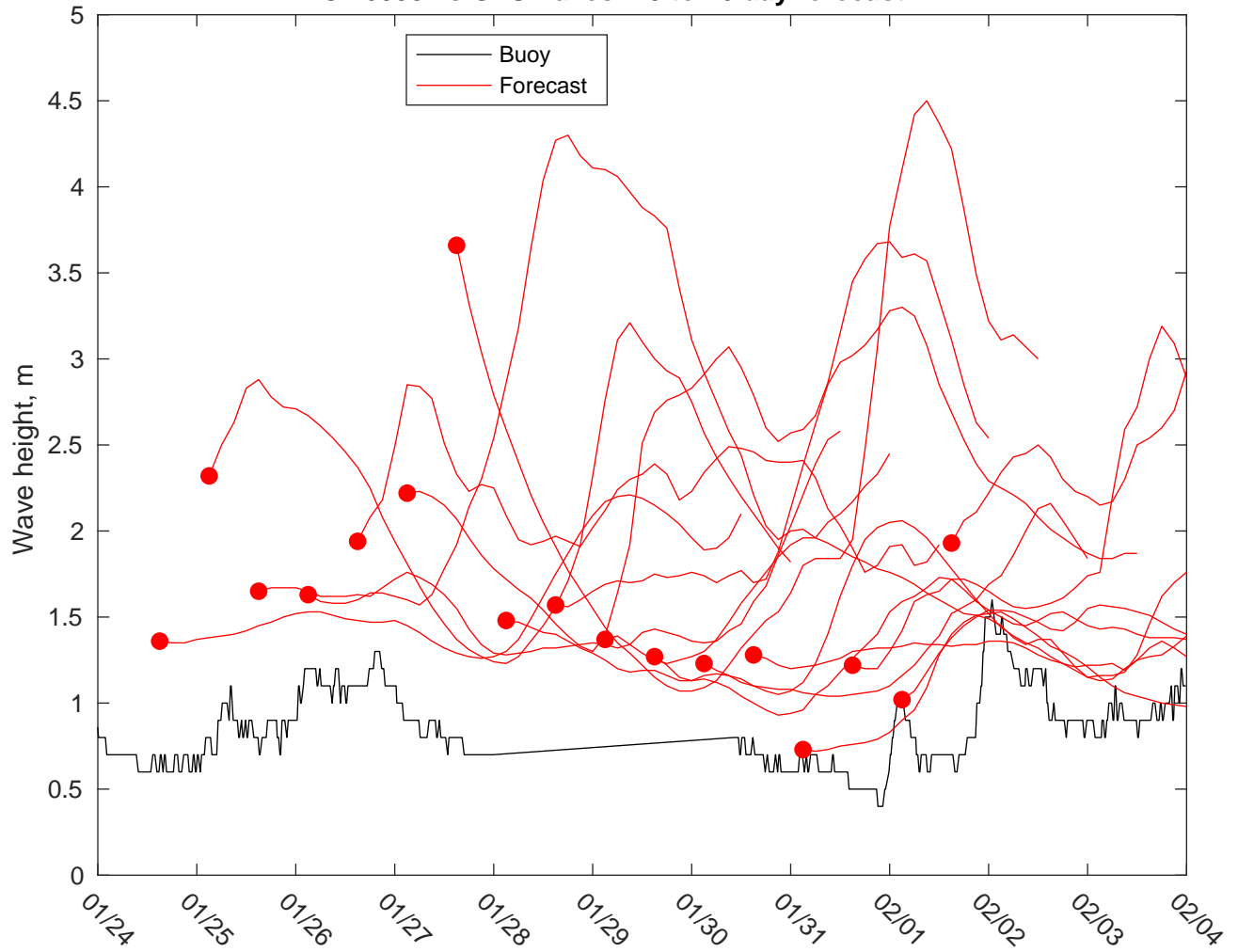
NDBC 46053 vs GFSWaves: 10 to 16 day forecast
