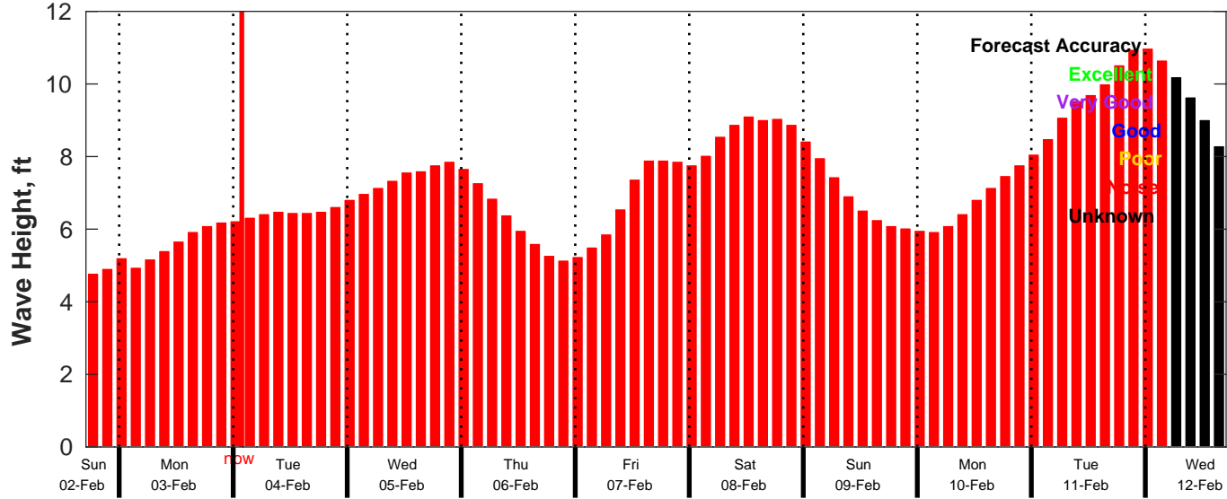
CMEMS Wave Forecast for NDBC 46053 from 02-Feb-2025 17:00:00 to 12-Feb-2025 17:00:00
