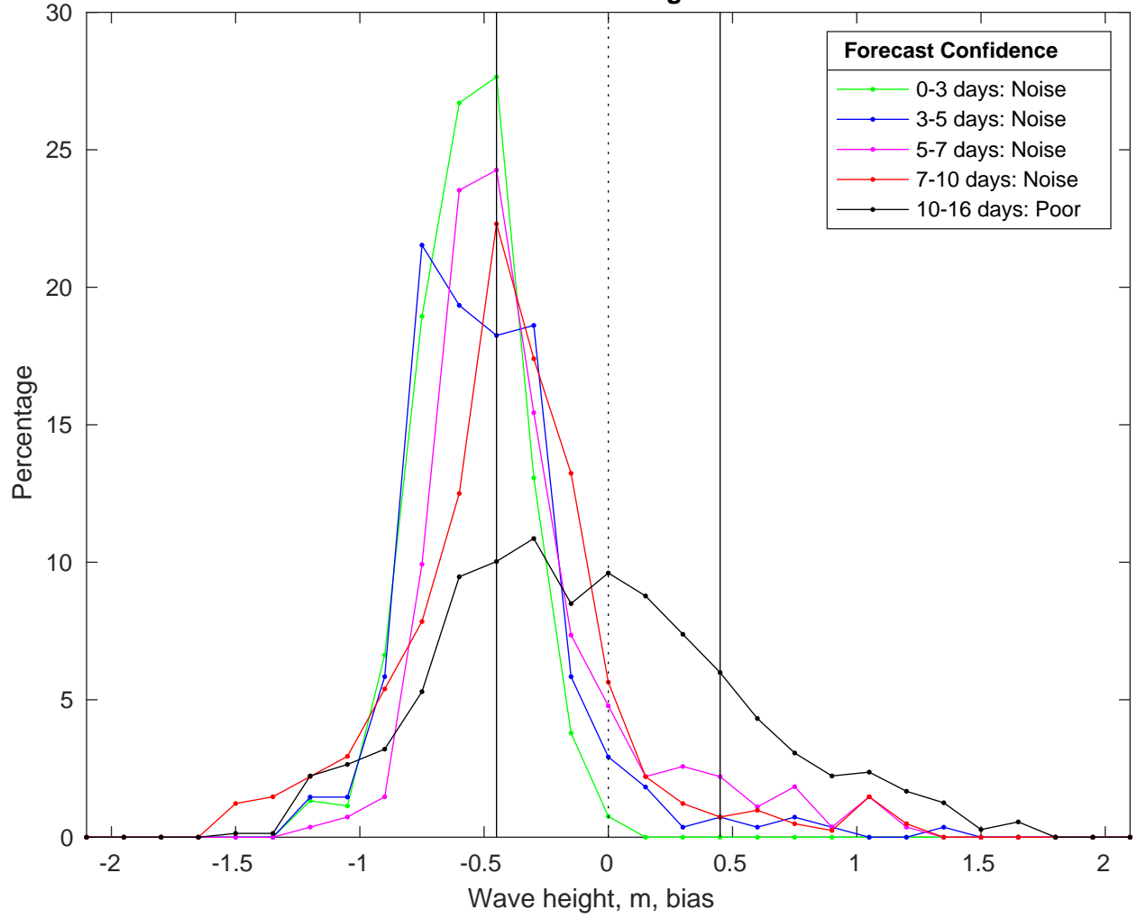
NDBC 46054 vs GFSWaves Bias Histogram: 04-Feb-2025
