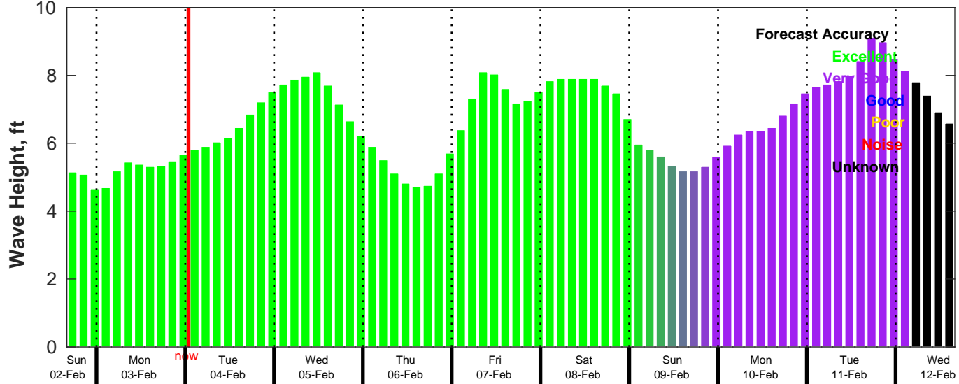
CMEMS Wave Forecast for NDBC 46054 from 02-Feb-2025 16:00:00 to 12-Feb-2025 16:00:00
