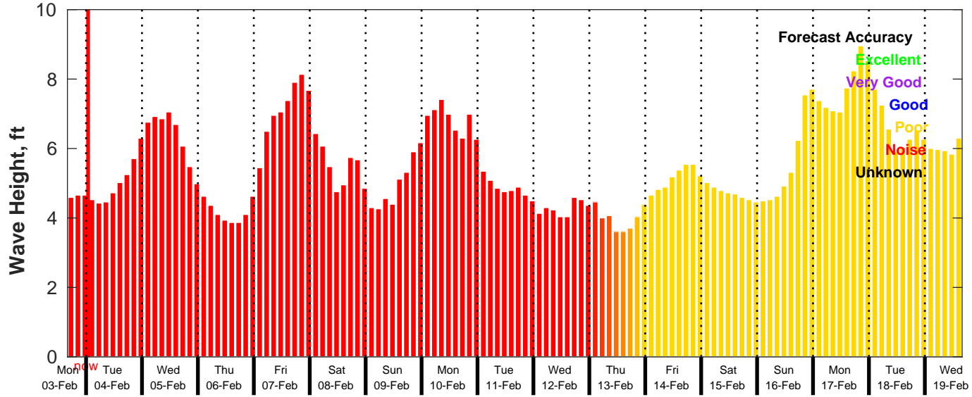
GFS Wave Forecast for NDBC 46054 from 03-Feb-2025 16:00:00 to 19-Feb-2025 16:00:00
