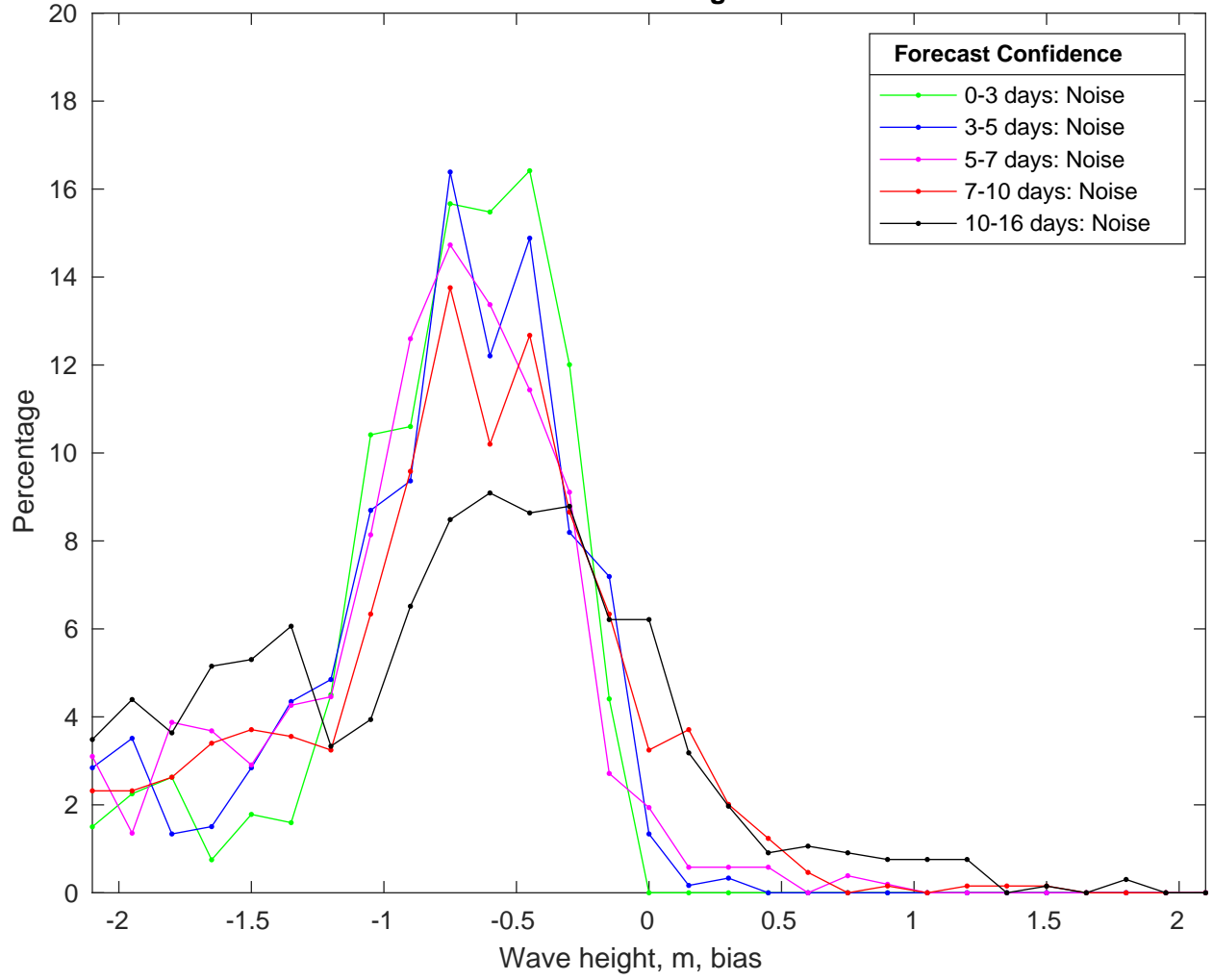
NDBC 46054 vs GFSWaves Bias Histogram: 26-Dec-2024
