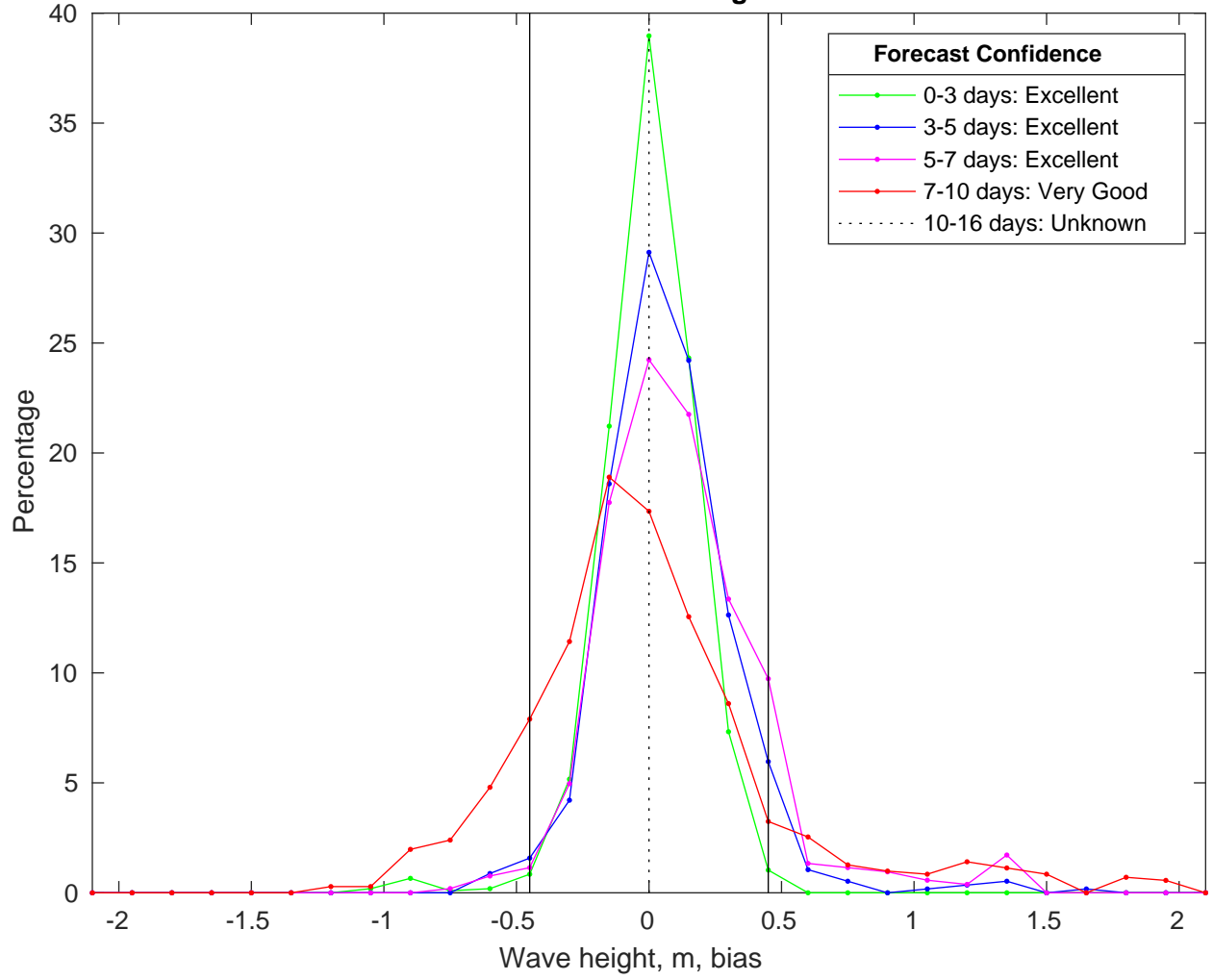
NDBC 46069 vs CMEMSWaves Bias Histogram: 04-Feb-2025
