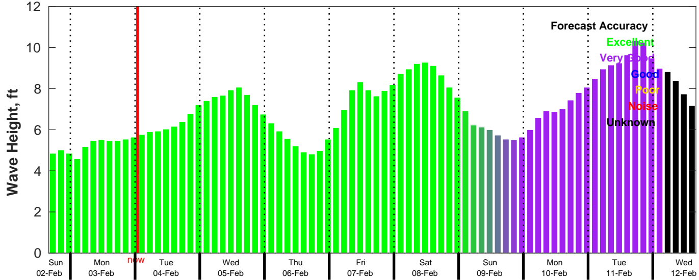
CMEMS Wave Forecast for NDBC 46069 from 02-Feb-2025 16:00:00 to 12-Feb-2025 16:00:00
