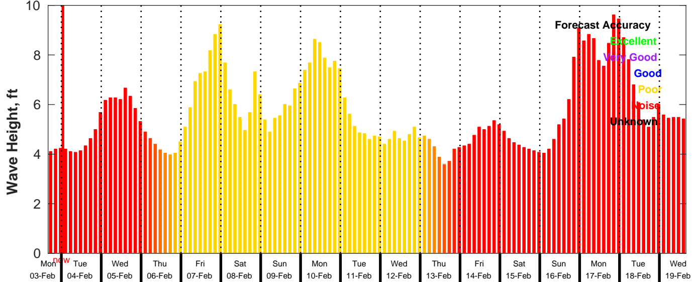
GFS Wave Forecast for NDBC 46069 from 03-Feb-2025 16:00:00 to 19-Feb-2025 16:00:00
