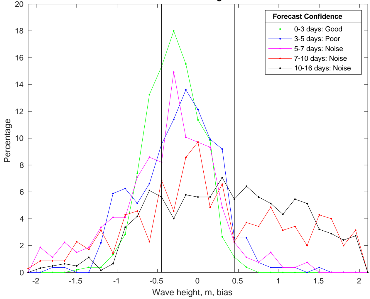
NDBC 46246 vs GFSWaves Bias Histogram: 04-Feb-2025
