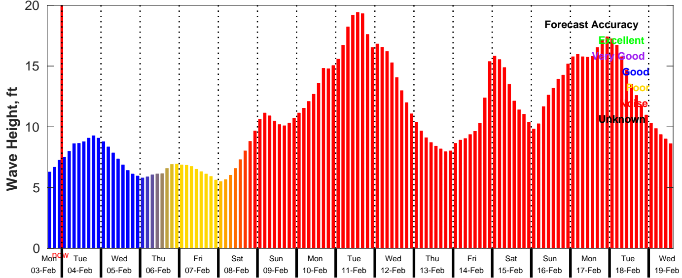
GFS Wave Forecast for NDBC 46246 from 03-Feb-2025 15:00:00 to 19-Feb-2025 15:00:00
