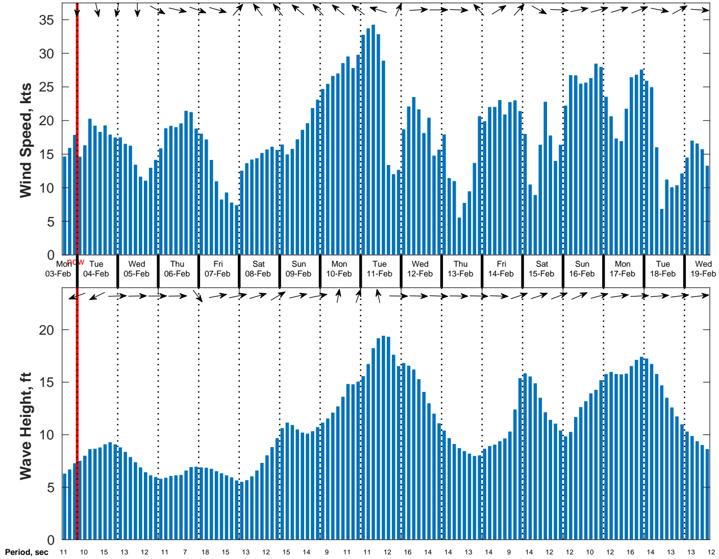
Wind & Wave Forecast for NDBC 46246 from 03-Feb-2025 15:00:00 to 19-Feb-2025 15:00:00
