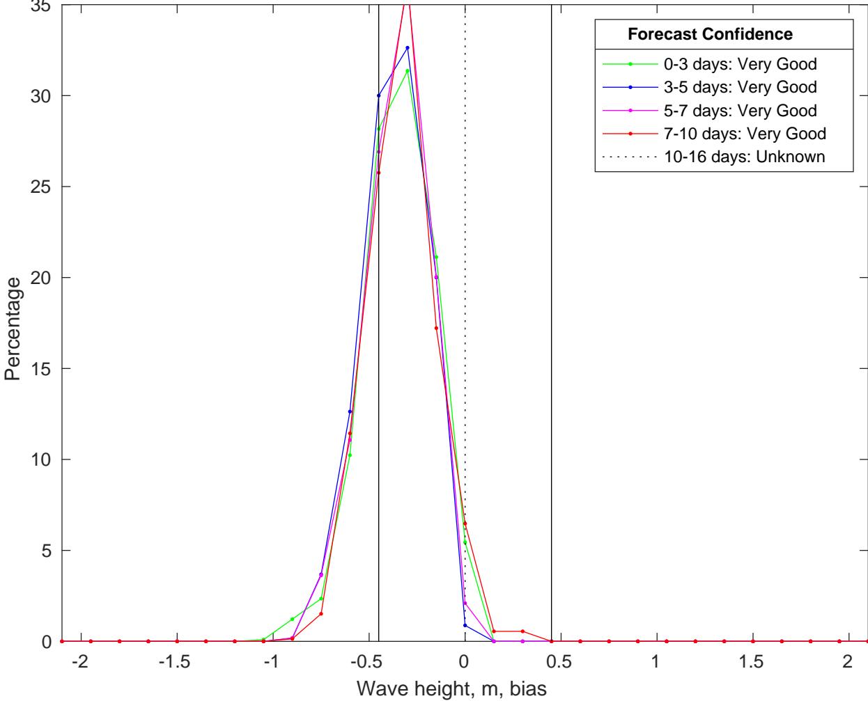
NDBC 51209 vs CMEMSWaves Bias Histogram: 04-Feb-2025
