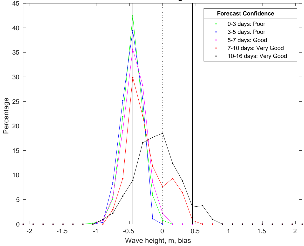
NDBC 51209 vs GFSWaves Bias Histogram: 04-Feb-2025
