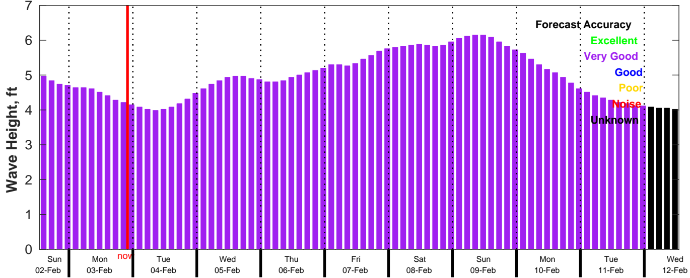
CMEMS Wave Forecast for NDBC 51209 from 02-Feb-2025 13:00:00 to 12-Feb-2025 13:00:00
