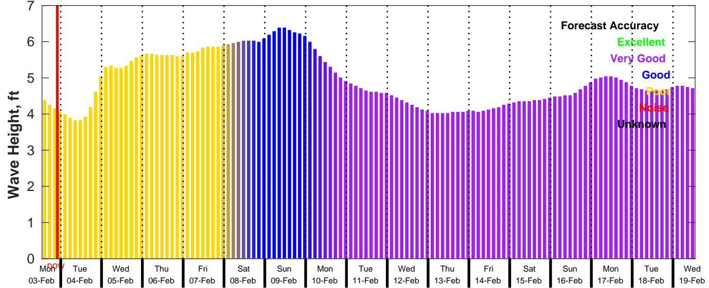
GFS Wave Forecast for NDBC 51209 from 03-Feb-2025 13:00:00 to 19-Feb-2025 13:00:00
