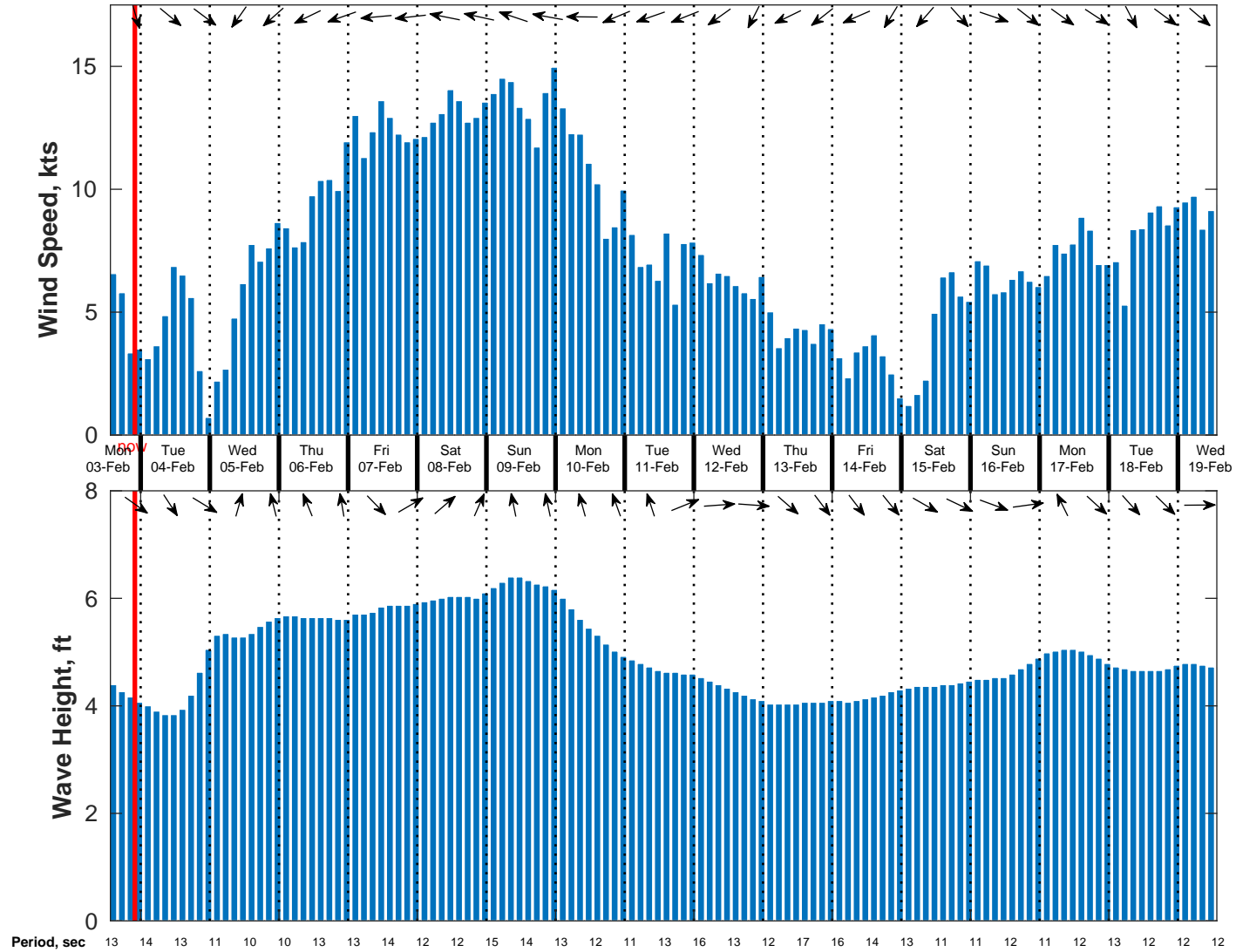
Wind & Wave Forecast for NDBC 51209 from 03-Feb-2025 13:00:00 to 19-Feb-2025 13:00:00
