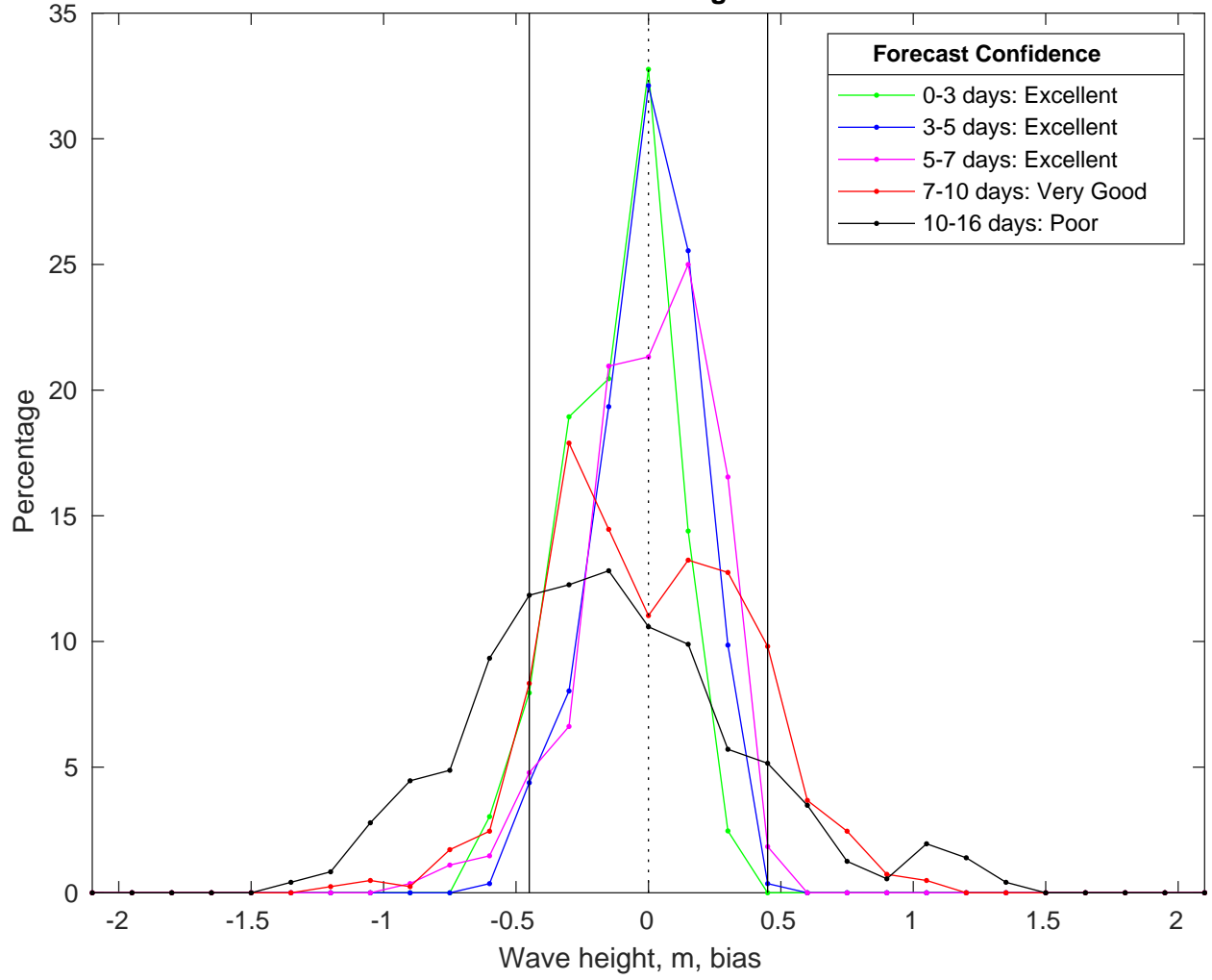
NDBC 52211 vs GFSWaves Bias Histogram: 04-Feb-2025
