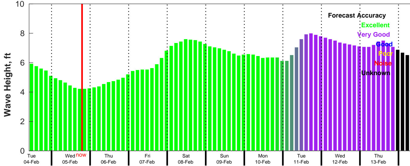
CMEMS Wave Forecast for NDBC 52211 from 03-Feb-2025 10:00:00 to 13-Feb-2025 10:00:00
