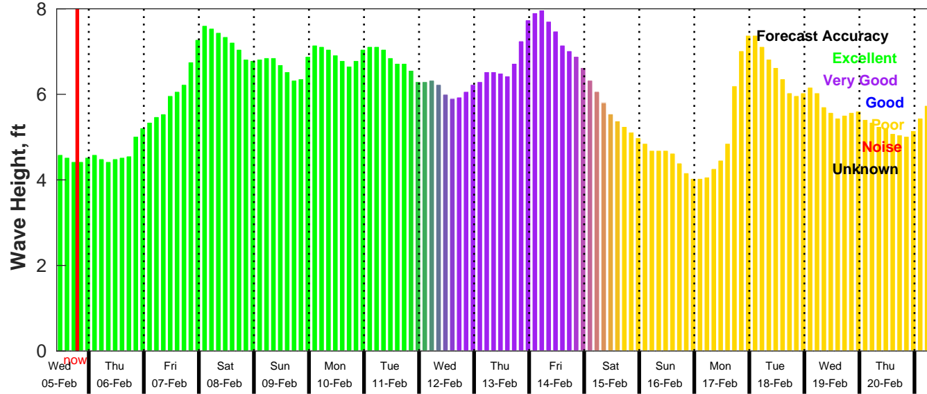
GFS Wave Forecast for NDBC 52211 from 04-Feb-2025 10:00:00 to 20-Feb-2025 10:00:00
