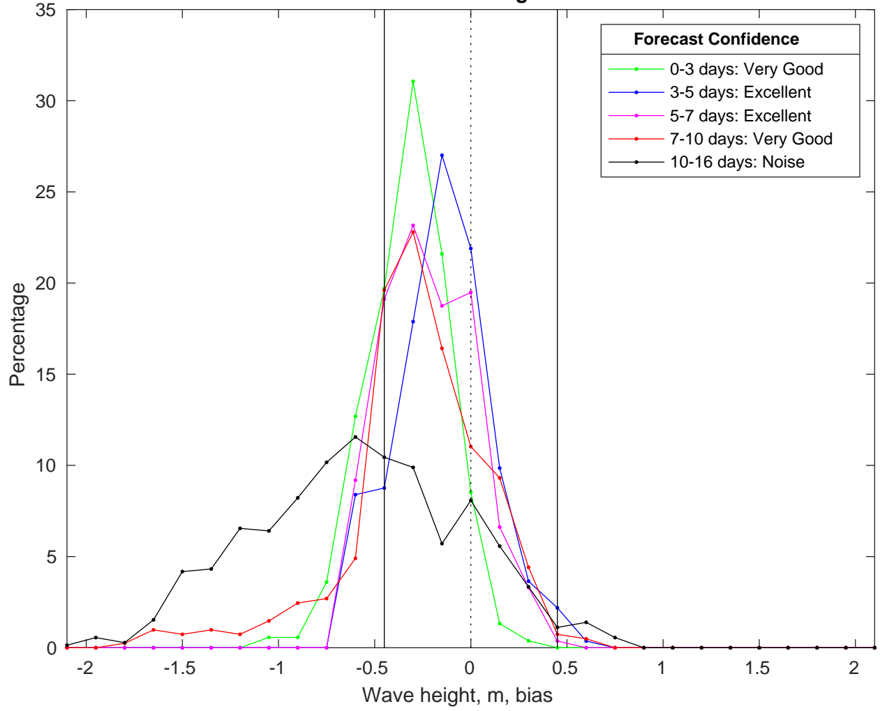
NDBC 52212 vs GFSWaves Bias Histogram: 04-Feb-2025
