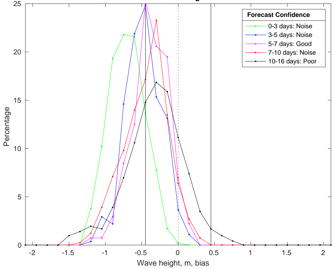
NDBC 52213 vs GFSWaves Bias Histogram: 04-Feb-2025
