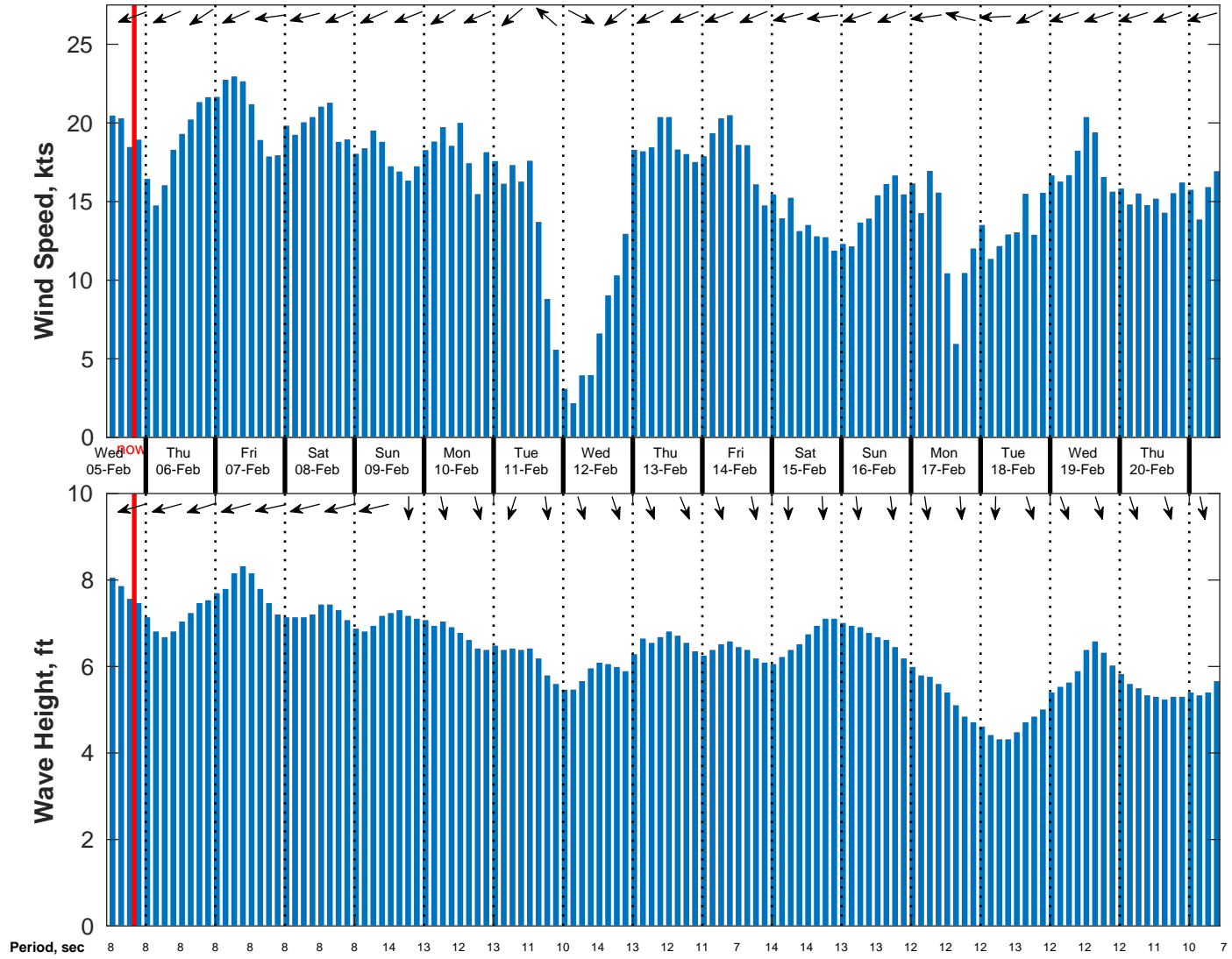
Wind & Wave Forecast for NDBC 52213 from 04-Feb-2025 11:00:00 to 20-Feb-2025 11:00:00
