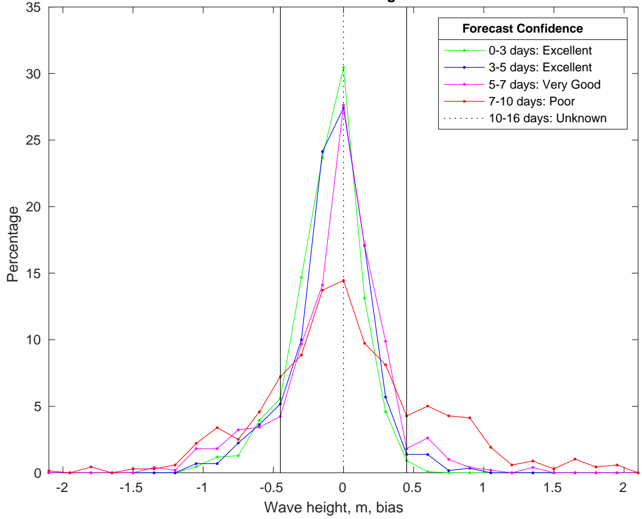
NDBC 41004 vs CMEMSWaves Bias Histogram: 05-Feb-2025
