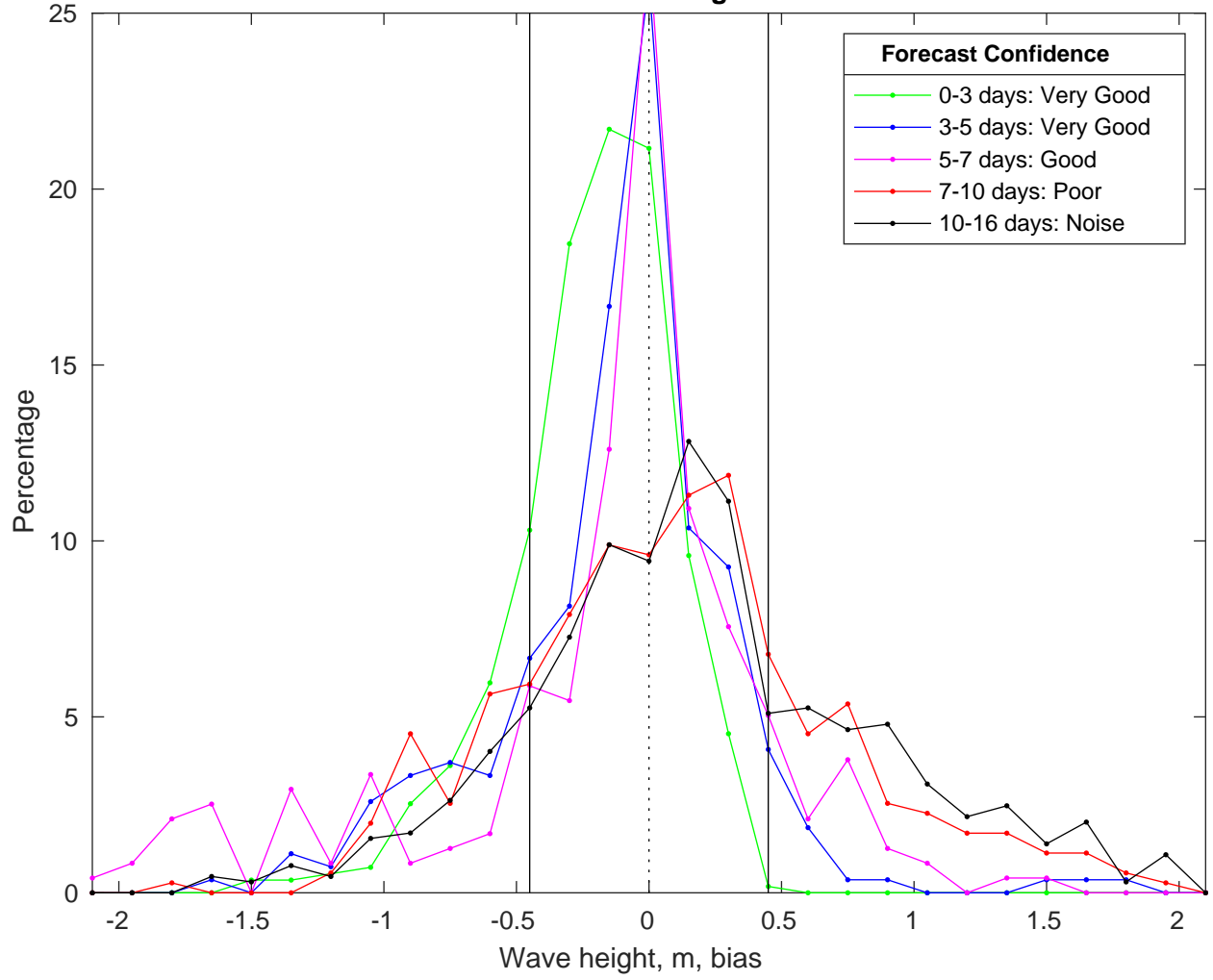
NDBC 41004 vs GFSWaves Bias Histogram: 05-Feb-2025
