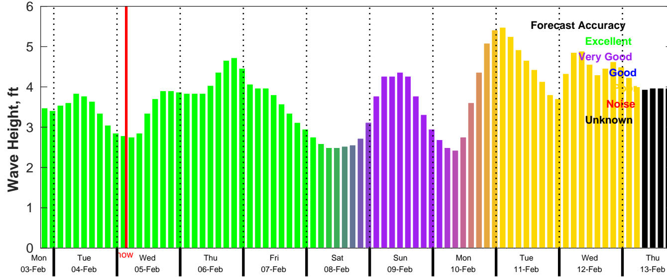
CMEMS Wave Forecast for NDBC 41004 from 03-Feb-2025 19:00:00 to 13-Feb-2025 19:00:00
