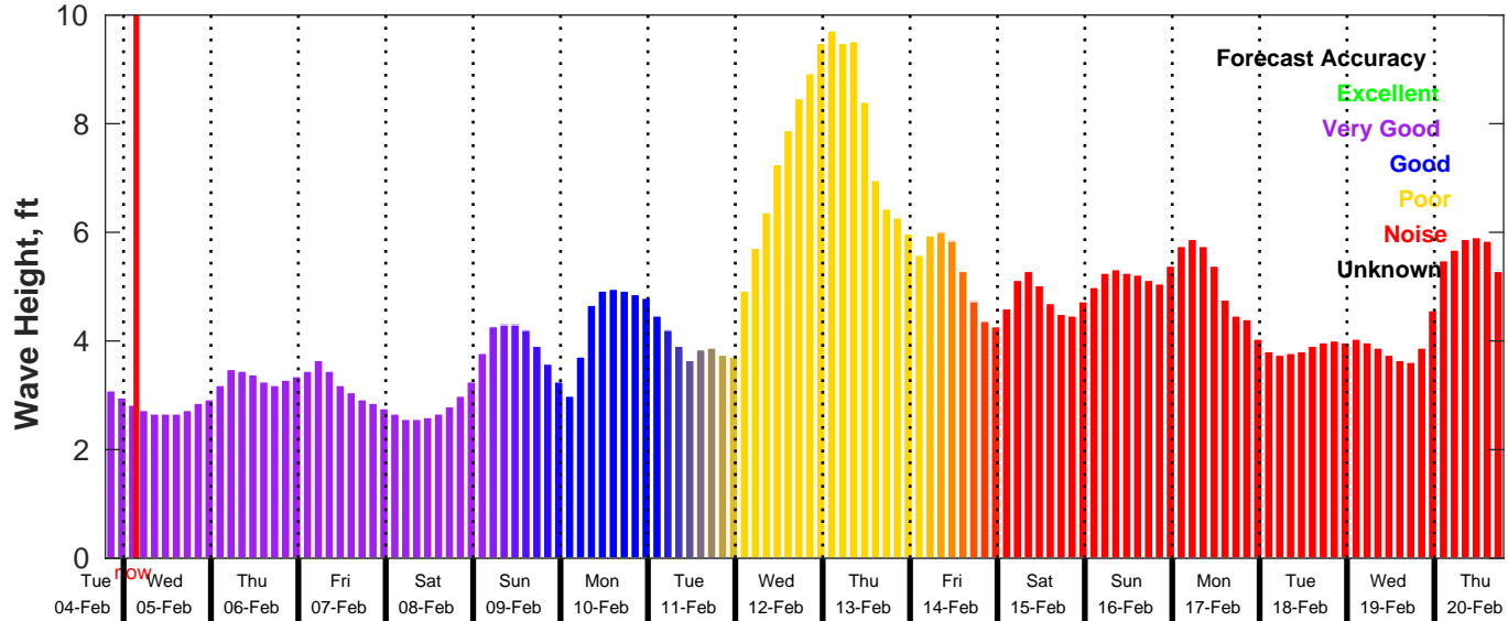
GFS Wave Forecast for NDBC 41004 from 04-Feb-2025 19:00:00 to 20-Feb-2025 19:00:00
