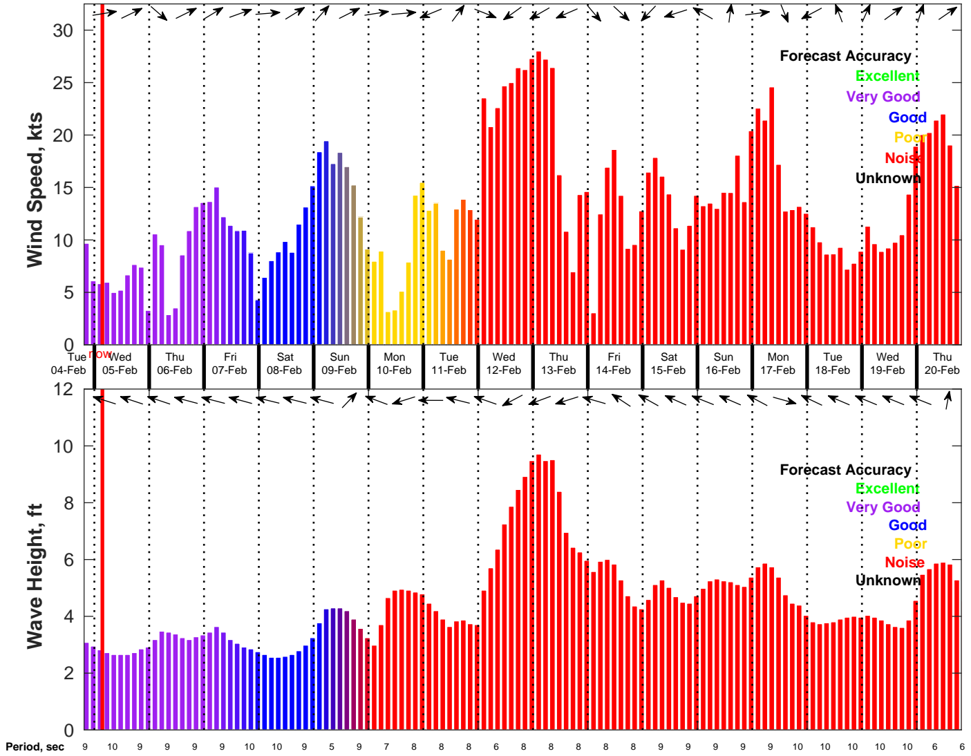
Wind & Wave Forecast for NDBC 41004 from 04-Feb-2025 19:00:00 to 20-Feb-2025 19:00:00
