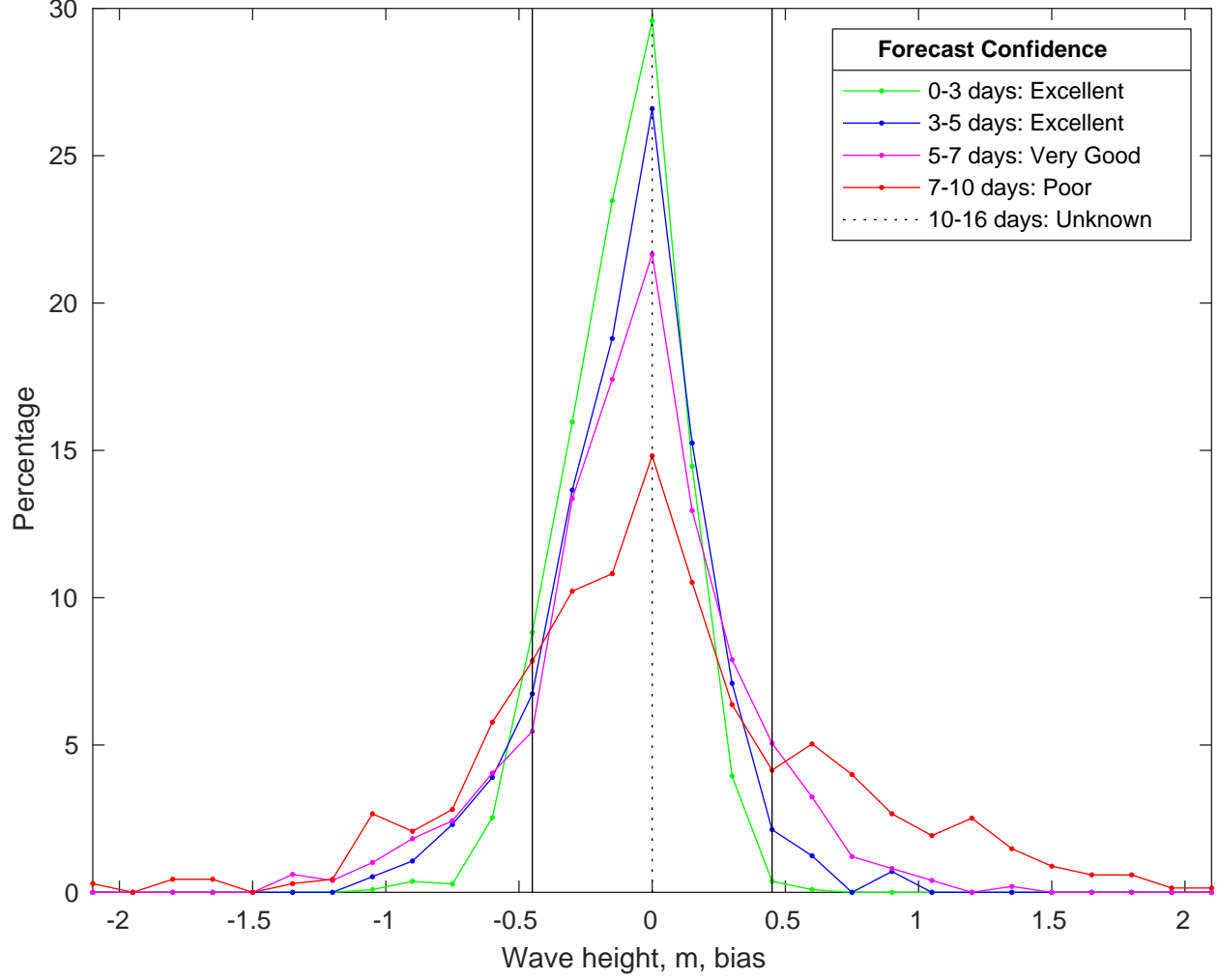
NDBC 41013 vs CMEMSWaves Bias Histogram: 05-Feb-2025
